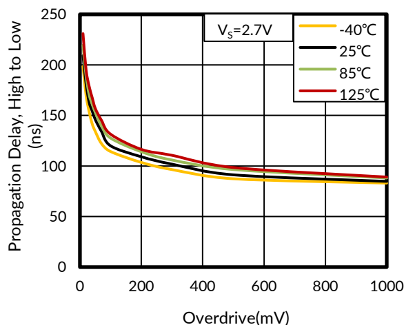
Figure 34. High to Low Propagation Delay vs Input Overdrive Voltage
