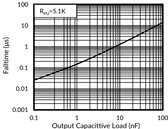
Figure 29. Falltime vs Capacitive Load
