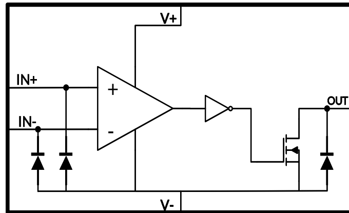
Figure 37. Functional Block Diagram
