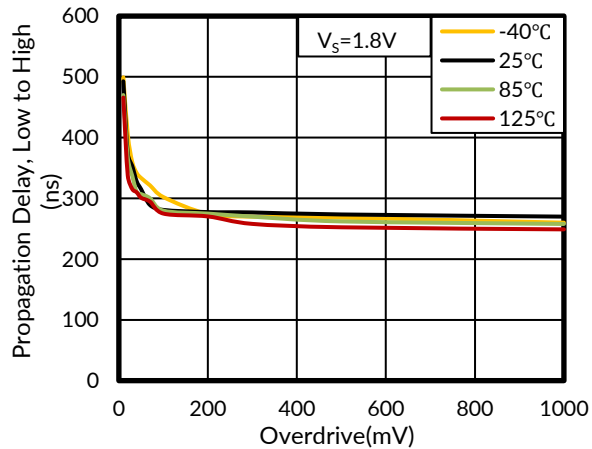
Figure 31. Low to High Propagation Delay vs Input Overdrive Voltage
