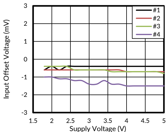
Figure 25. Input Offset Voltage vs Supply Voltage at -40^{\circ}\text{C}
