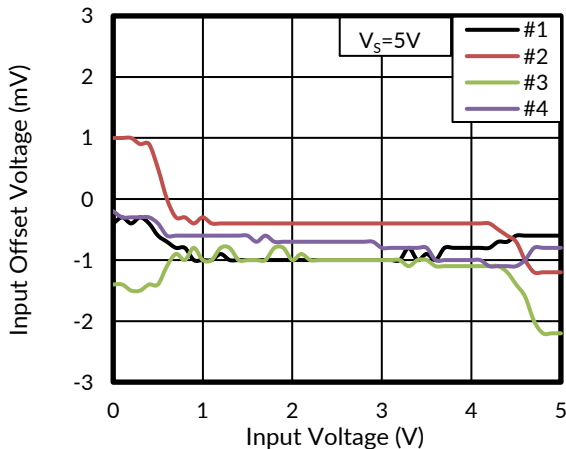
Figure 23. Offset Voltage vs Input Voltage at 85°C
