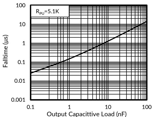
Figure 29. Falltime vs Capacitive Load
