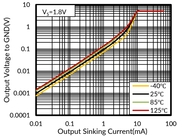
Figure 7. Output Voltage vs Output Sinking Current
