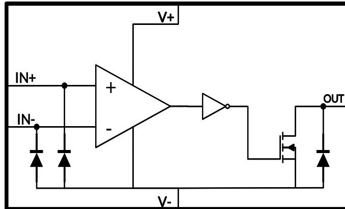
Figure 37. Functional Block Diagram
