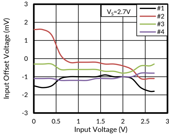
Figure 19. Offset Voltage vs Input Voltage at 85°C
