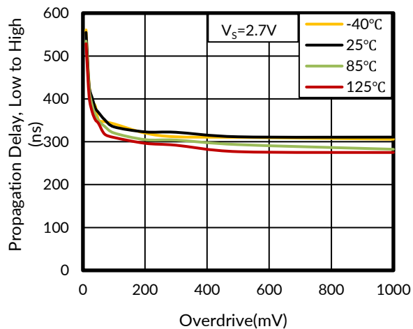
Figure 33. Low to High Propagation Delay vs Input Overdrive Voltage
