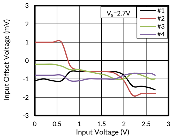
Figure 17. Offset Voltage vs Input Voltage at -40^\circ\text{C}
