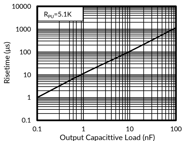
Figure 30. Risettime vs Capacitive Load
