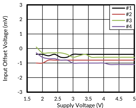
Figure 27. Input Offset Voltage vs Supply Voltage at 85^{\circ}\text{C}
