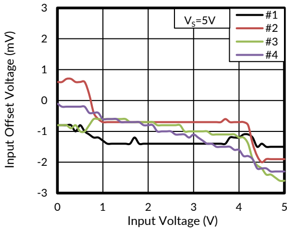
Figure 21. Offset Voltage vs Input Voltage at -40°C
