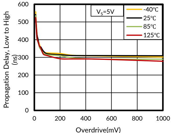
Figure 35. Low to High Propagation Delay vs Input Overdrive Voltage
