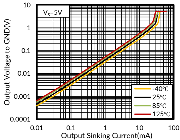
Figure 9. Output Voltage vs Output Sinking Current
