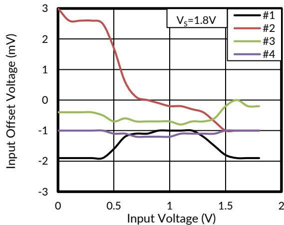
Figure 15. Offset Voltage vs Input Voltage at 85^\circ\text{C}
