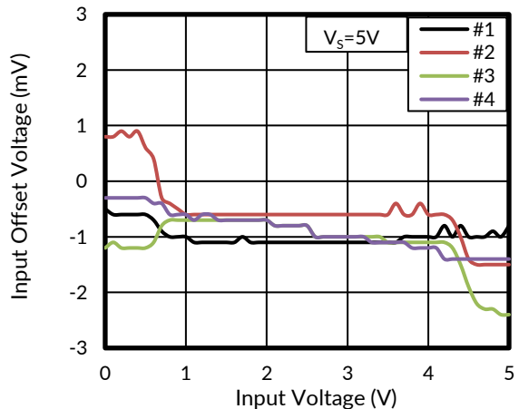
Figure 22. Offset Voltage vs Input Voltage at 25°C
