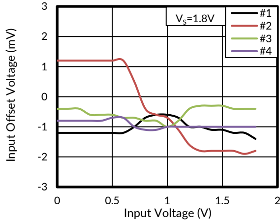
Figure 13. Offset Voltage vs Input Voltage at -40^\circ\text{C}
