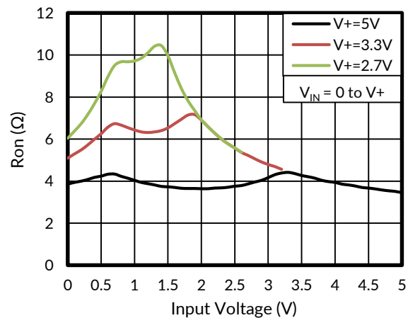
Figure 6. Typical Ron as a Function of Input Voltage
