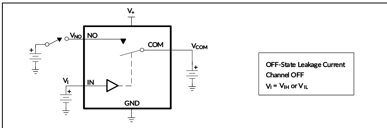
Figure 11. OFF-State Leakage Current ( I_{com(off)} , I_{no(off)} )
