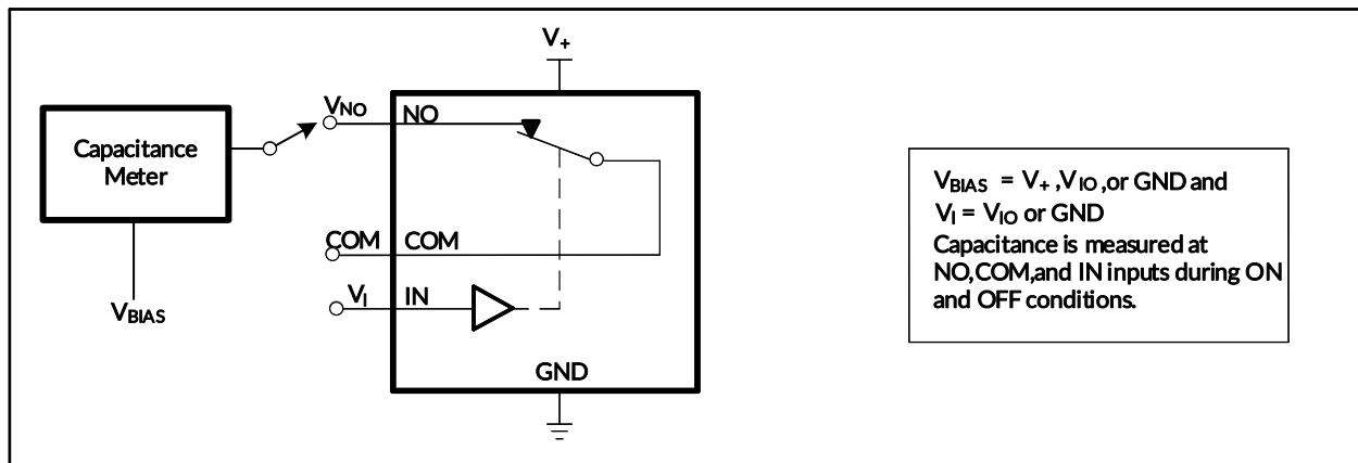
Figure 13. Capacitance ( C_I , C_{COM(OFF)} , C_{COM(ON)} , C_{NO(OFF)} , C_{NO(ON)} )
