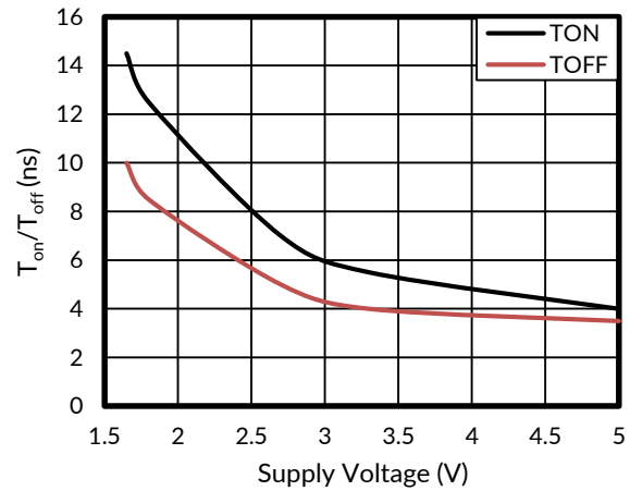
Figure 8. T_{on} and T_{off} vs Supply Voltage
