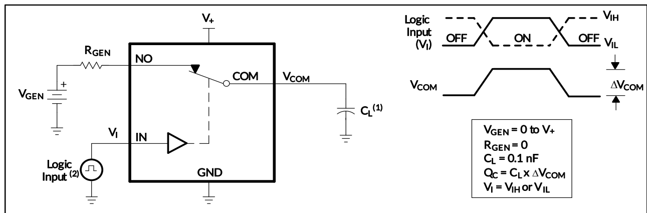
Figure 21. Charge Injection ( Q_C )
