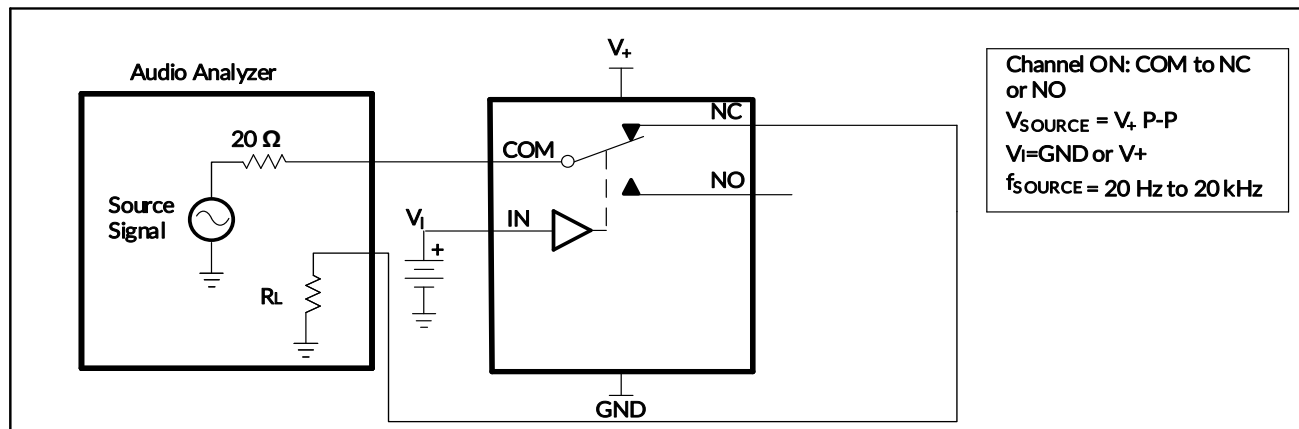
Figure 22. Total Harmonic Distortion (THD)
