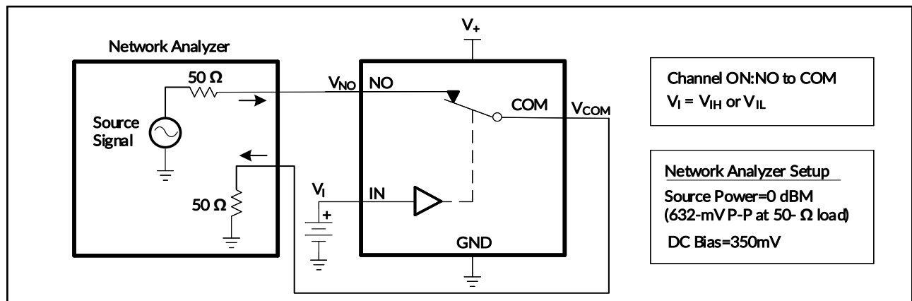
Figure 18. Bandwidth (BW)
