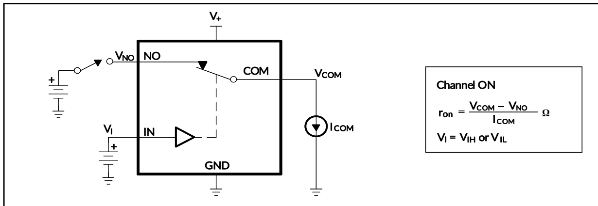
Figure 10. ON-State Resistance ( R_{on} )
