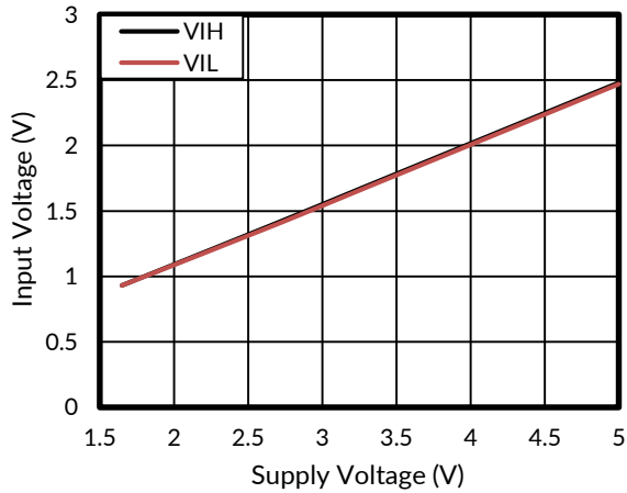
Figure 9. Logic-Level Threshold vs V_{+}
