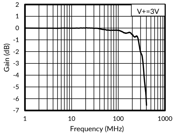
Figure 3. Bandwidth vs Frequency
