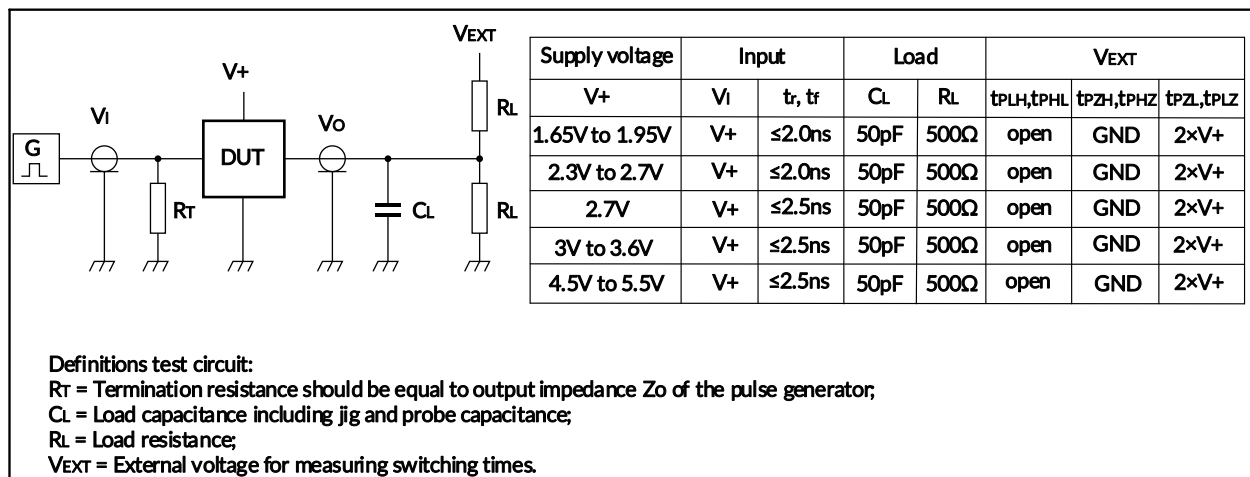
Figure 14. Test circuit for measuring switching times
