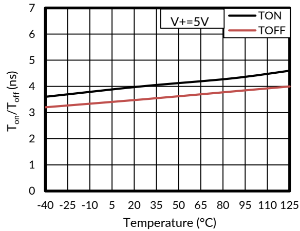
Figure 7. T_{on} and T_{off} vs Temperature
