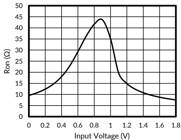
Figure 5. Typical Ron as a Function of Input Voltage ( V_+ = 1.8\text{ V} )
