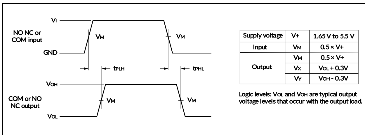
Figure 15. Propagation delay ( t_{pd} )
