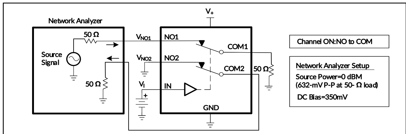
Figure 20. Crosstalk ( X_{TALK} )
