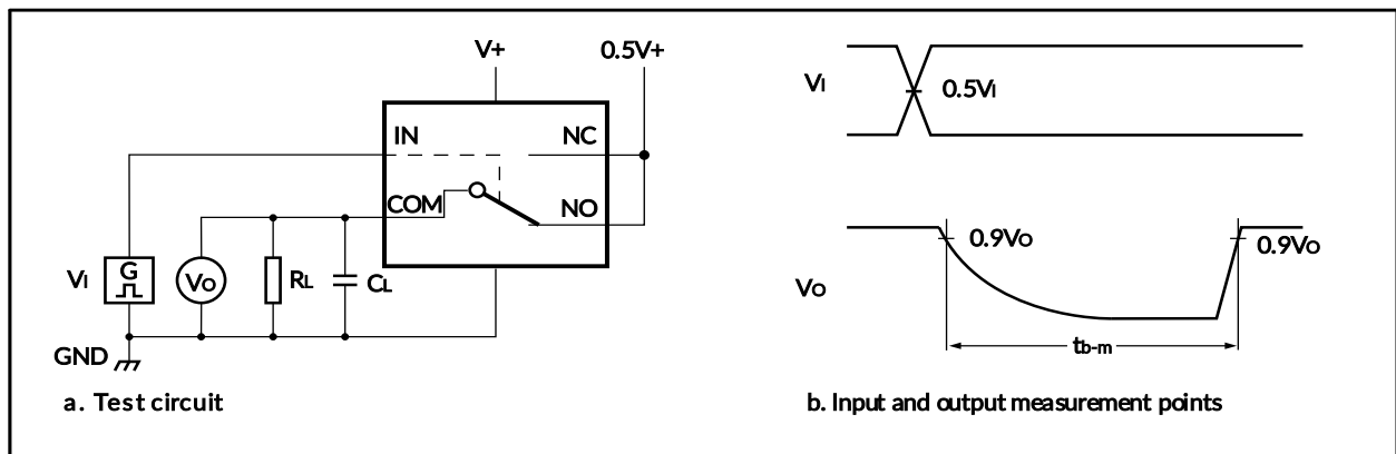
Figure 17. Break-Before-Make Time ( t_{BBM} )
