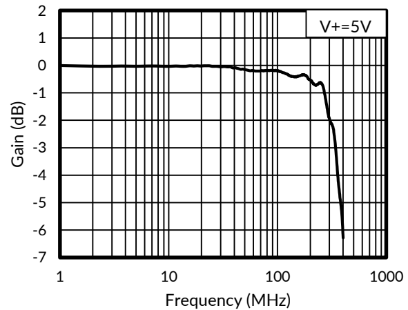
Figure 4. Bandwidth vs Frequency
