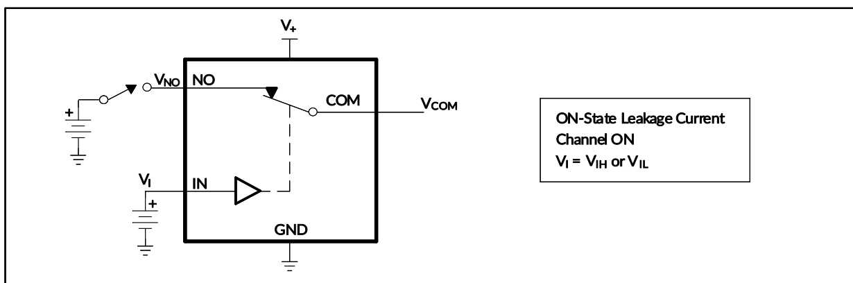
Figure 12. ON-State Leakage Current ( I_{com(on)} , I_{no(on)} )
